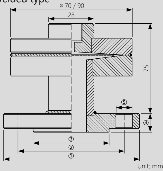
Welded type
