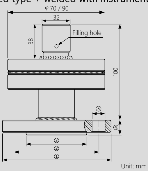
Welded type + welded with instrument
