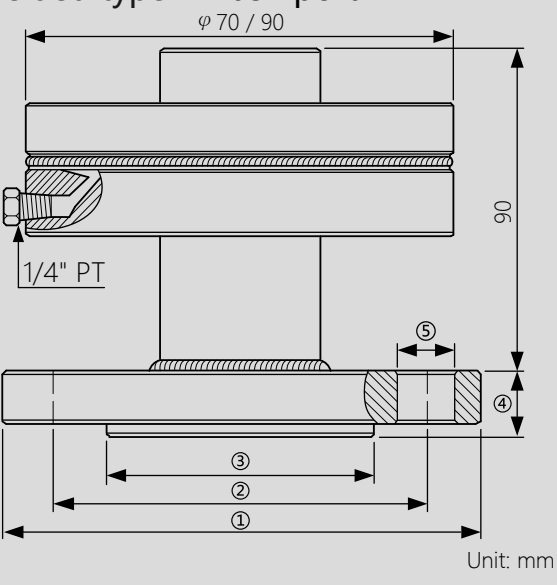
Welded type + flush port
