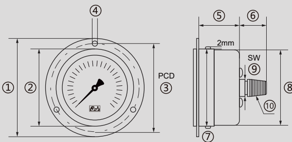
Center back mount with flange (black iron case and chromium plated bayonet ring)
