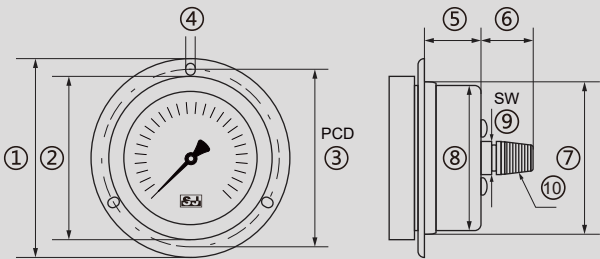
Center back mount with flange (all chromium plated case)
